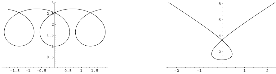
Figure 4: The generating curves of a parabolic surfaces with \kappa_1 = m\kappa_2 + n and n + m - 1 > 0 . We consider in (a) the subcase m < n + 1 , with m = 1 and n = 2 . In (b) we show the subcase m \geq n + 1 with m = 3 and n = 1 .
