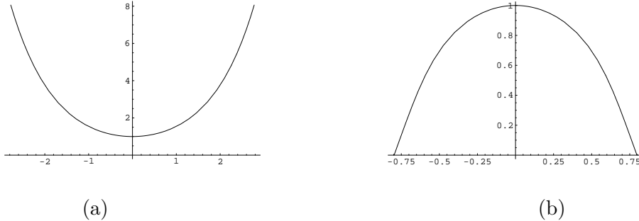
Figure 5: The generating curves of a parabolic surfaces with \kappa_1 = m\kappa_2 + n . We consider in (a) the case n + m - 1 > 0 and subcase m \geq n + 1 , with m = 2 and n = 0 . In (b), we show the case n + m - 1 < 0 with m = -2 and n = 1 .
